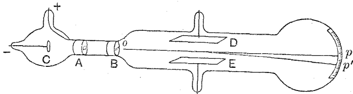
FIG. 14. Thomson's apparatus for cathode rays
